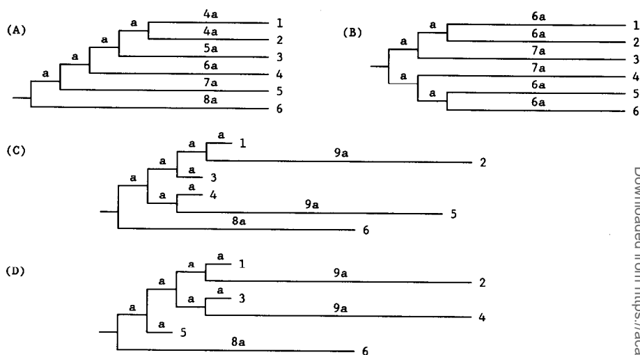
FIG. 3.—Four model trees used for computer simulation. These trees are identical with those used by Saitou and Imanishi (1989).
