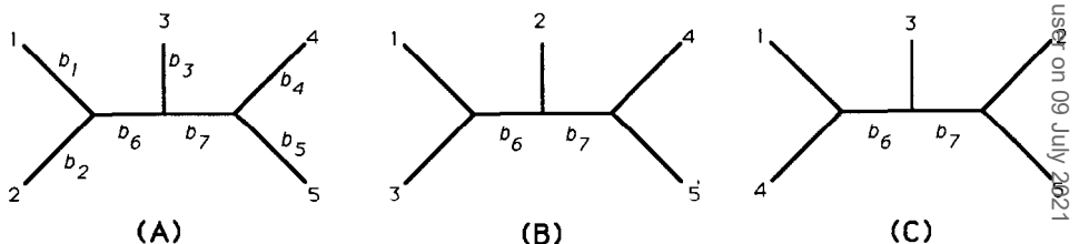
FIG. 2.—Hypothetical trees illustrating computation of branch lengths and S values
