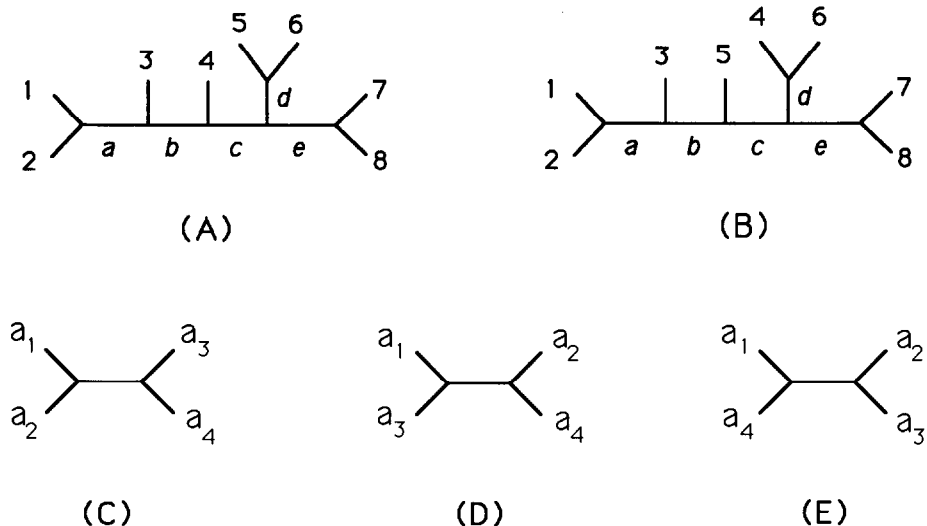
FIG. 1.—Hypothetical trees illustrating various computations discussed in text
