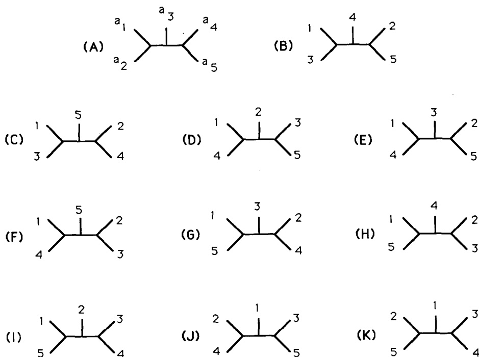
FIG. A1.—(A), Five groups of sequences ( a_1 , a_2 , a_3 , a_4 , and a_5 ) associated with two contiguous interior branches. The rearrangement of the five groups of sequences generates 10 different topologies [(B)–(K)] with d_T = 4 .
