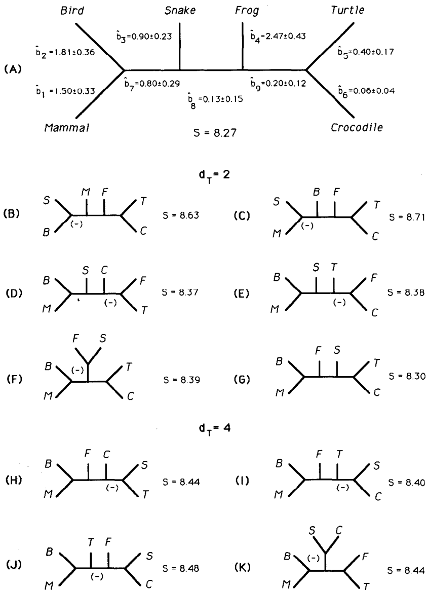
FIG. 4.—NJ tree (A) and its closely related trees (B–K) for the 18S rRNA genes from six tetrapod species [mammals (M), birds (B), snakes (S), frogs (F), turtles (T), and crocodiles (C)]. The estimates of branch lengths (i.e., \hat{b} \times 100 ) and their standard errors were obtained by the least-squares method. The estimate of the length of a branch with a (–) sign was negative. The S value in this figure represents the true value multiplied by 100.
